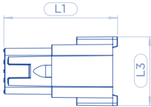
Male plug
