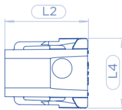
Female plug
